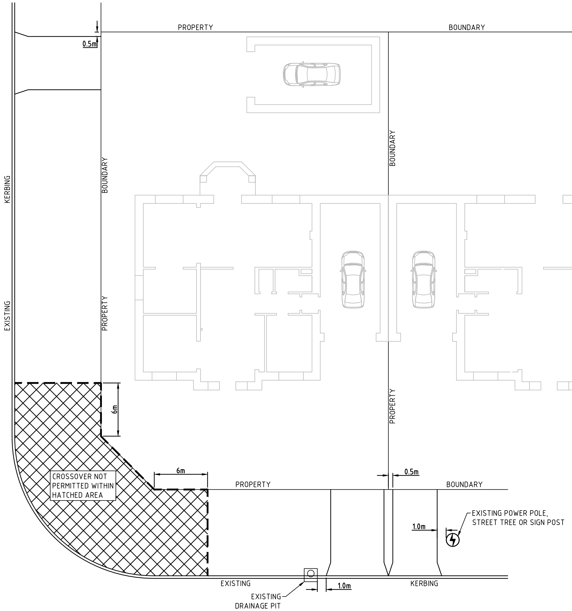
CROSSOVER LOCATION PLAN SCALE 1:250
